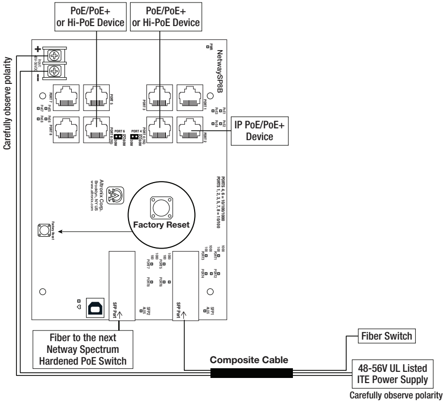
Fig. 6 - NetWaySP8WPN – Typical Application with Composite Cable
